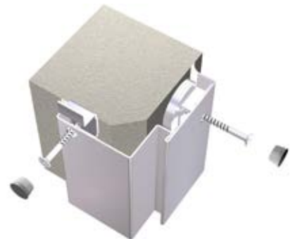
STEEL CASING 24 PROFILE Corner casing Retrofit (renovation)
